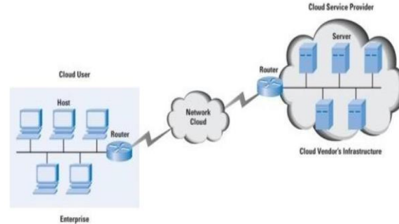
fig. 1 cloud architecture
