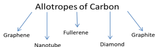
Figure1: Carbonallotropesexamples
