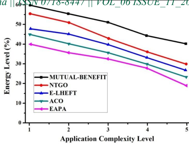
Figure 3: Application complexity level Vs Energy level
