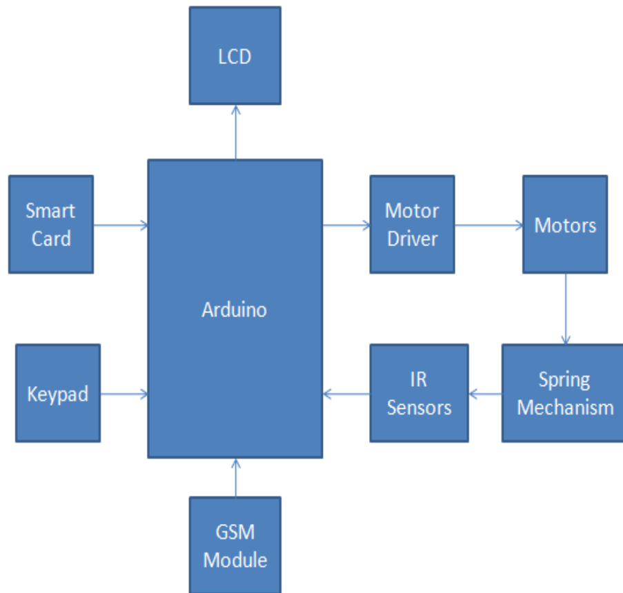
Fig 1 :block diagram
