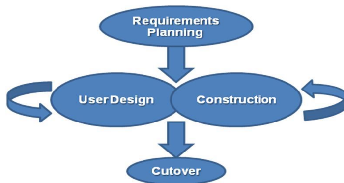
Figure 2. Methodology
