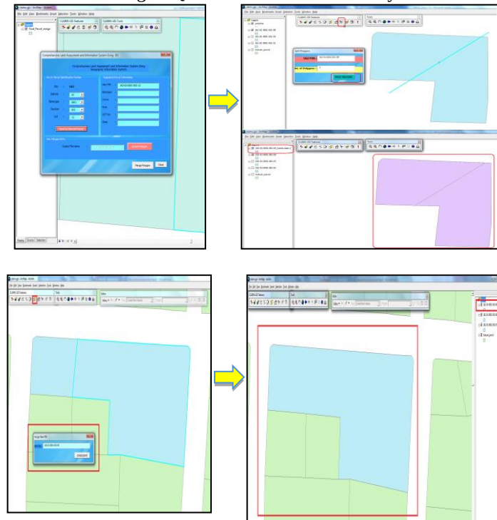
Figure 4. Subdivision/Consolidation Program
