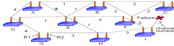
Fig. 1. Multi-radio WMN
