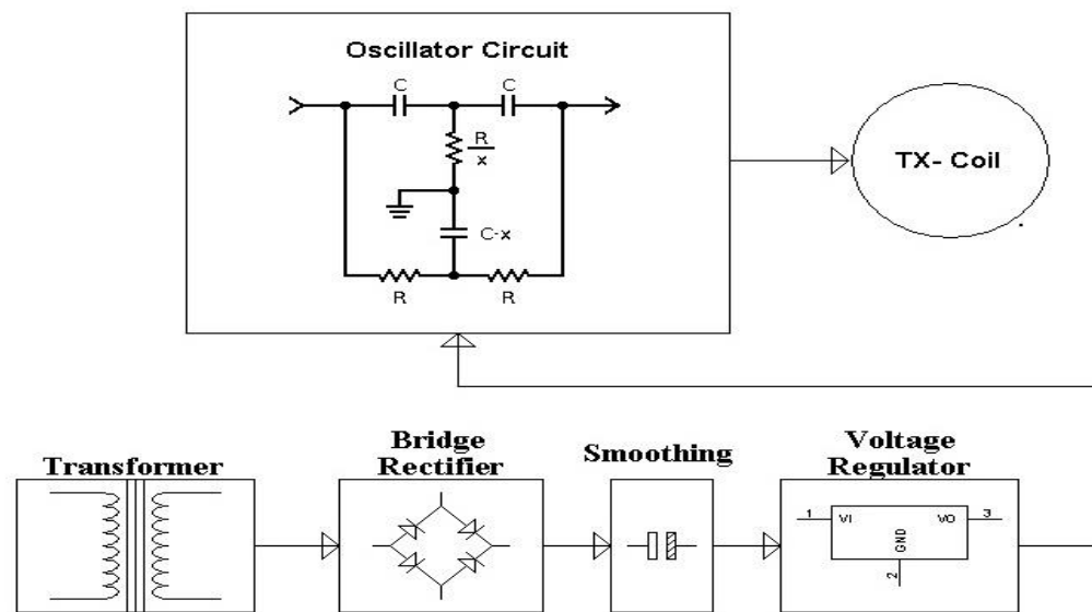
Fig : Transfer circuit
