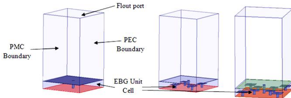
Figure 2: Simulation setup for measurement of coefficient of reflection for three EBG models
