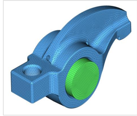
Figure 4: Mesh Model
