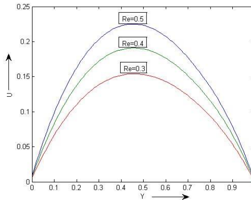
Fig.1. Velocity profile for different values of variable of transpiration Reynolds numbers ( Re ) viscosity parameter
