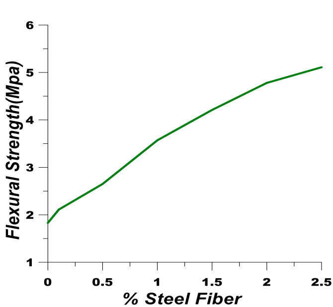
Fig. 10 Flexural Strength Test
