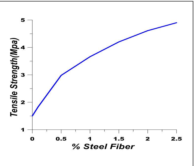
Fig. 5 Tensile Strength Test
