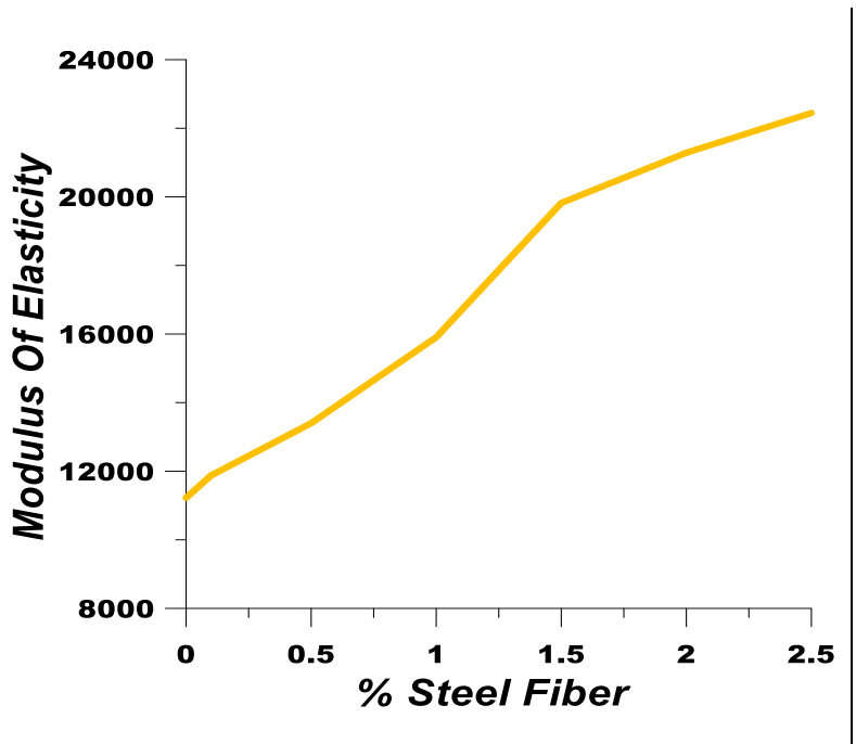
Fig. 7 Modulus Of Elasticity Test
