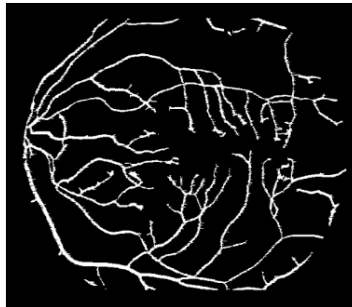
Figure 4.SVM Model Prediction
