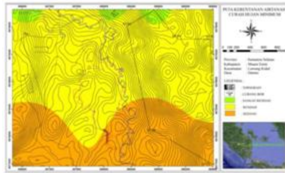
Figure 4. Groundwater Vulnerability on Minimum Rainfall Map
