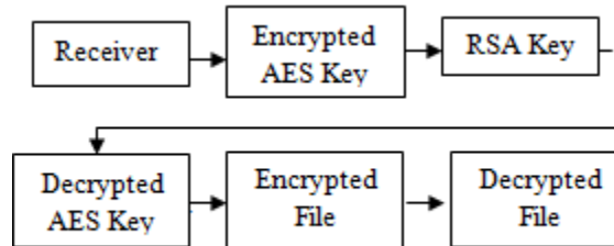
Figure 6: Receiver Process Model
