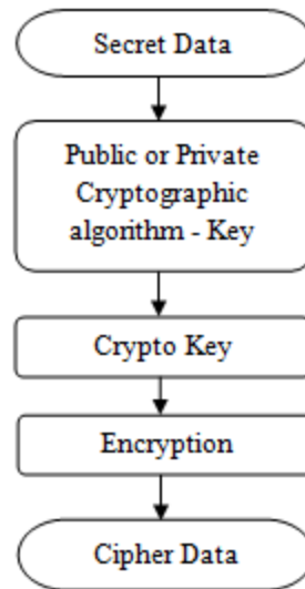
Figure 1: Usual Encryption
