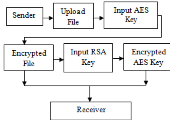
Figure 5: Sender Process Model
