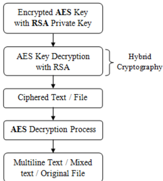
Figure 4: Decryption Flow Model in HTSecure Approach
