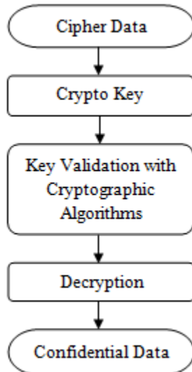
Figure 2: Usual Decryption
