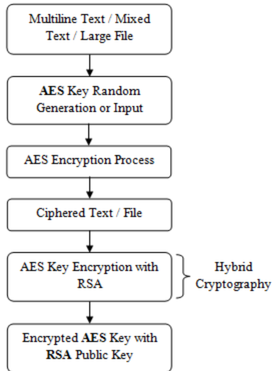
Figure 3: Encryption Flow Model in HTSecure Approach
